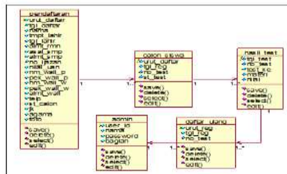
Gambar 13. Class Diagram
