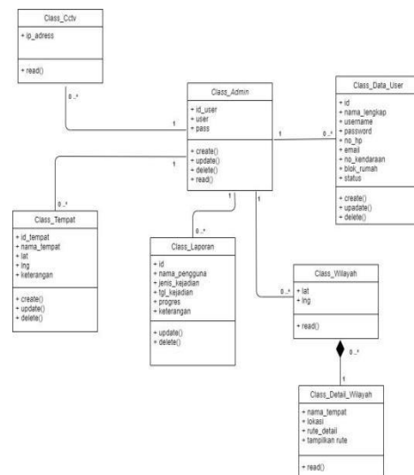
Gambar 5. Class Diagram Server Admin
